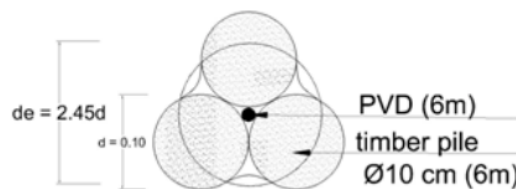
Figure-2. Schematic design of Hybrid pile.
