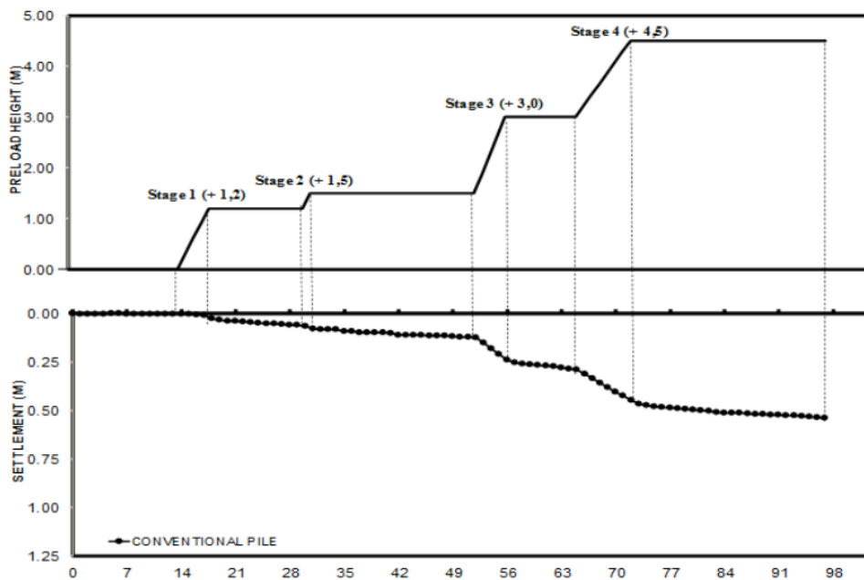
Figure-7. Settlement observation of conventional pile reinforcement.
