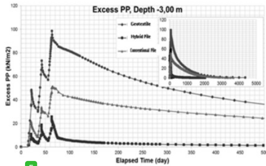
5 Figure-13. Excess pore water depth 3.0 meters.
