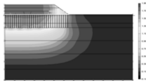
Figure-12. Shading deformation Hybrid pile reinforcement.
