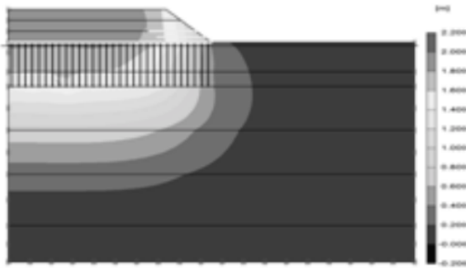
Figure-11. Shading deformation conventional pile reinforcement.
