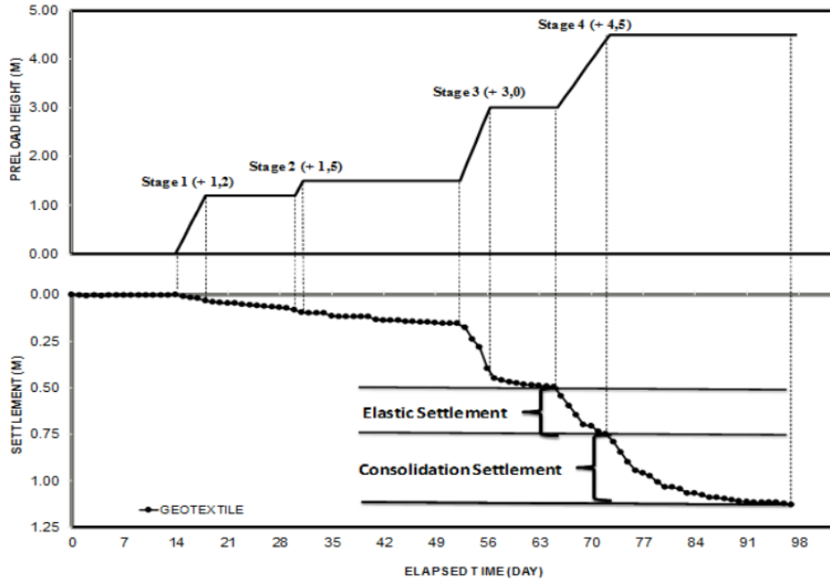
Figure-6. Settlement observation of geotextile reinforcement.
