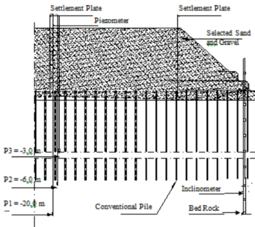
Figure-4. Conventional pile reinforcement.
