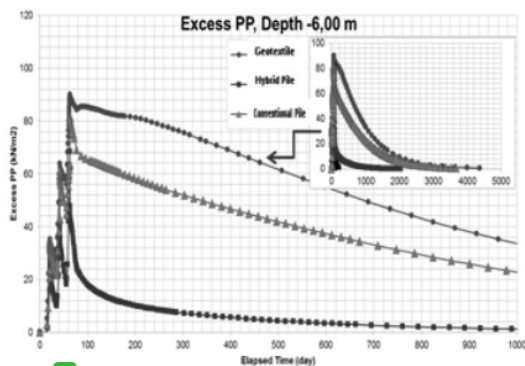
5 Figure-14. Excess pore water depth 6.0 meters.
