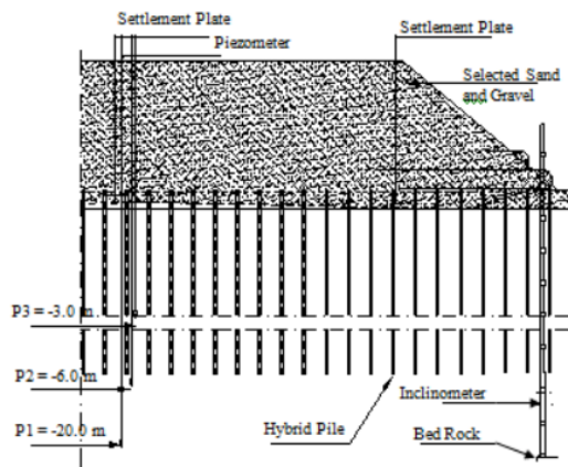
Figure-5. Hybrid pile reinforcement.
