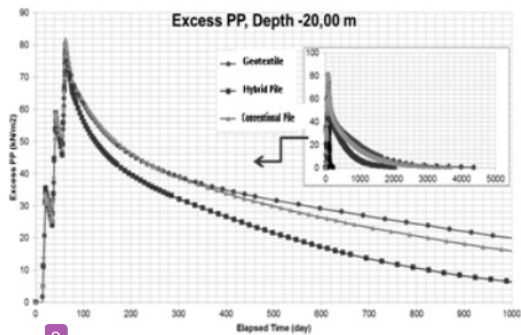
9 Figure-15. Excess pore water depth 20.0 meters.
