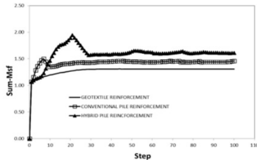
Figure-16. Safety factor.
